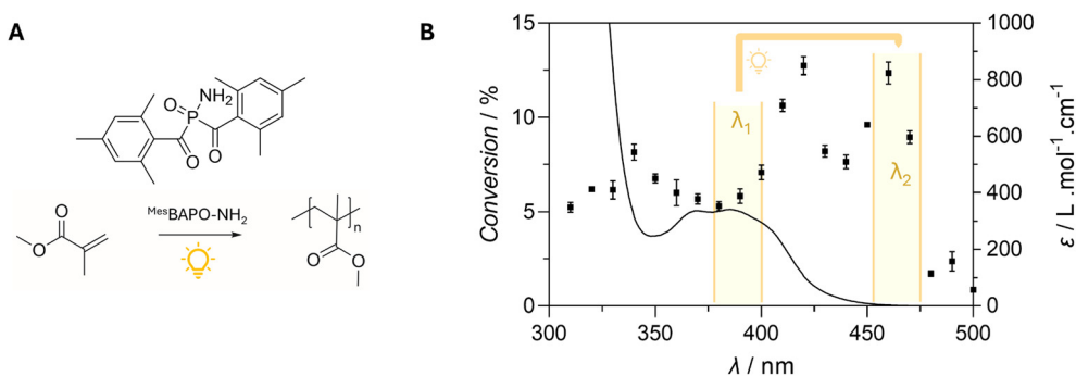
Fig. 2 (A) Photopolymerization of methyl methacrylate (MMA) initiated by the photo-initiator Mes BAPO-NH 2 ( C PI = 5 mmol L -1 ), (B) photochemical action plot of the photopolymerization illustrating that the monomer conversion is higher in a wavelength regime where the absorption is very low. The yellow arrow indicates that the highest reactivities can be obtained at the far red-edge, where the extinction is minimal, thus offering a key opportunity for deep penetration with high reactivities. Solutions were irradiated with 6.02 \times 10^{19} photons at each wavelength. Refer to the first and third section of the ESI† for the calculations related to the provided example and the experimental data related to the recording of the photochemical action plot, respectively.
