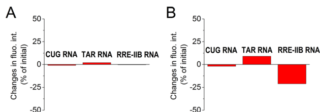
Fig. 2 Structures of the CUG RNA, HIV-1 TAR RNA and HIV-1 RRE-IIB RNA oligonucleotides used in this study and changes in the fluorescence intensity (in % of the initial intensity) of aurones ( A ) 2a and ( B ) 1d ( c_{\text{lig}} = 5 \mu\text{M} ) in the presence of 1 equiv. of each RNA oligonucleotide in a buffer (pH = 7); positive values indicate fluorescence light-up in the presence of RNA and negative values indicate fluorescence quenching in the presence of RNA. The fluorescence output was measured upon excitation at \lambda_{\text{ex}} = 350 nm for 2a and at \lambda_{\text{ex}} = 450 nm for 1d . To ensure the reproducibility, each measurement was repeated at least three times, and the repeat experiments gave values within 20%.
