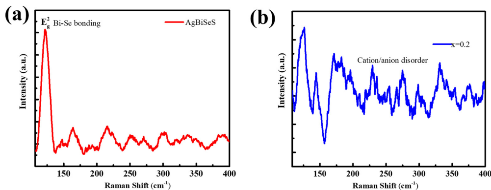
Fig. 2 (a) Room-temperature Raman spectra of AgBiSeS and (\text{AgBiSeS})_{0.8}(\text{PbSe})_{0.2} illustrating how the increase in the configurational entropy aids in disorder in the system, which eventually evades the Raman peak.
