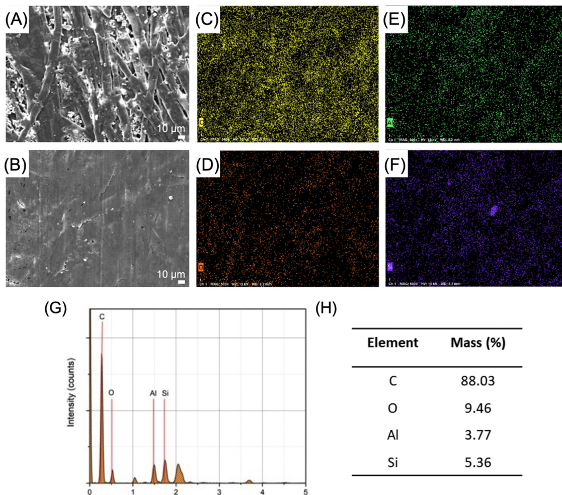
Fig. 3 Morphology and elemental composition of the PoP device surface: SEM images of the surface morphology of the paper (A) before and (B) after applying the graphite trace (by drawing). Trace analysis of the four main elements: (C) carbon, (D) oxygen, (E) aluminium, and (F) silicon on the graphite surface. (G) and (H) Analysis of element composition and quantification of the major elements on the graphite surface.
