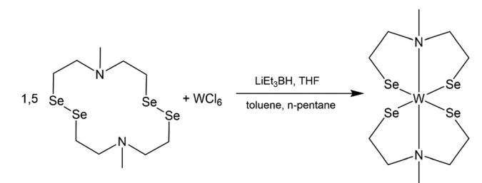
Scheme 1 Reaction of cyclic selenium containing ligand [(SeC 2 H 4 ) 2 NMe 2 ] 2 with tungsten hexachloride (WCl 6 ) to the desired complex [W{(SeC 2 H 4 ) 2 NMe 2 }] 2 .
