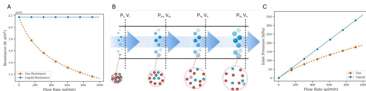
Fig. 1: (A) Comparing resistance of a straight channel for an incompressible liquid and a compressible gas as a function of flow rate. (B) Schematic for flow of gas through a straight channel. Density varies with
