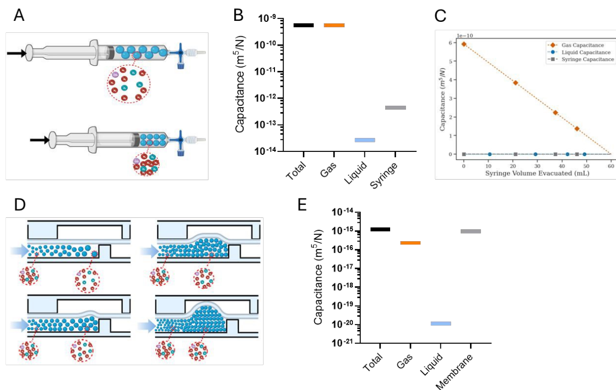
Fig. 2: (A) Schematic for the source of capacitance in a syringe. Theoretically, the compressibility of gas and the flexibility of the syringe material both contribute. (B) Total capacitance, and the individual contributions of fluid compressibility and syringe material deformability to it, varying with pressure within the syringe through one pressurization cycle. Data is plotted as boxplots for capacitance at relative pressure from 5 to 10 kPa, demonstrating no visually identifiable variability of the data. (C) For a syringe filled with gas and for that filled with liquid, variation of the major contributor of total capacitance with changing volume of the syringe. (D) Schematic for pressurization of a microfluidic valve with gas. The compression of gas and deformation of the membrane can be modeled as capacitive components contributing to the total capacitance of a valve. (E) Plot for the total capacitance of a microfluidic valve, and the individual
