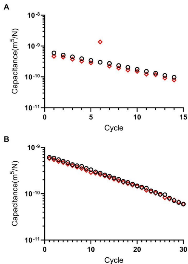
Fig. 5: Forced-air oscillator capacitance drops as syringe fluid volume is evacuated. As the syringe pump runs, and syringe fluid volume reduces, total (syringe and fluid) capacitance drops over time, or as presented here after each cycle of oscillations. A) 100 \mu\text{m} thick membrane and B) 20 \mu\text{m} membrane oscillator system. Oscillators were run at 500 and 200 \mu\text{L}/\text{min} respectively and a 60 mL syringe.
