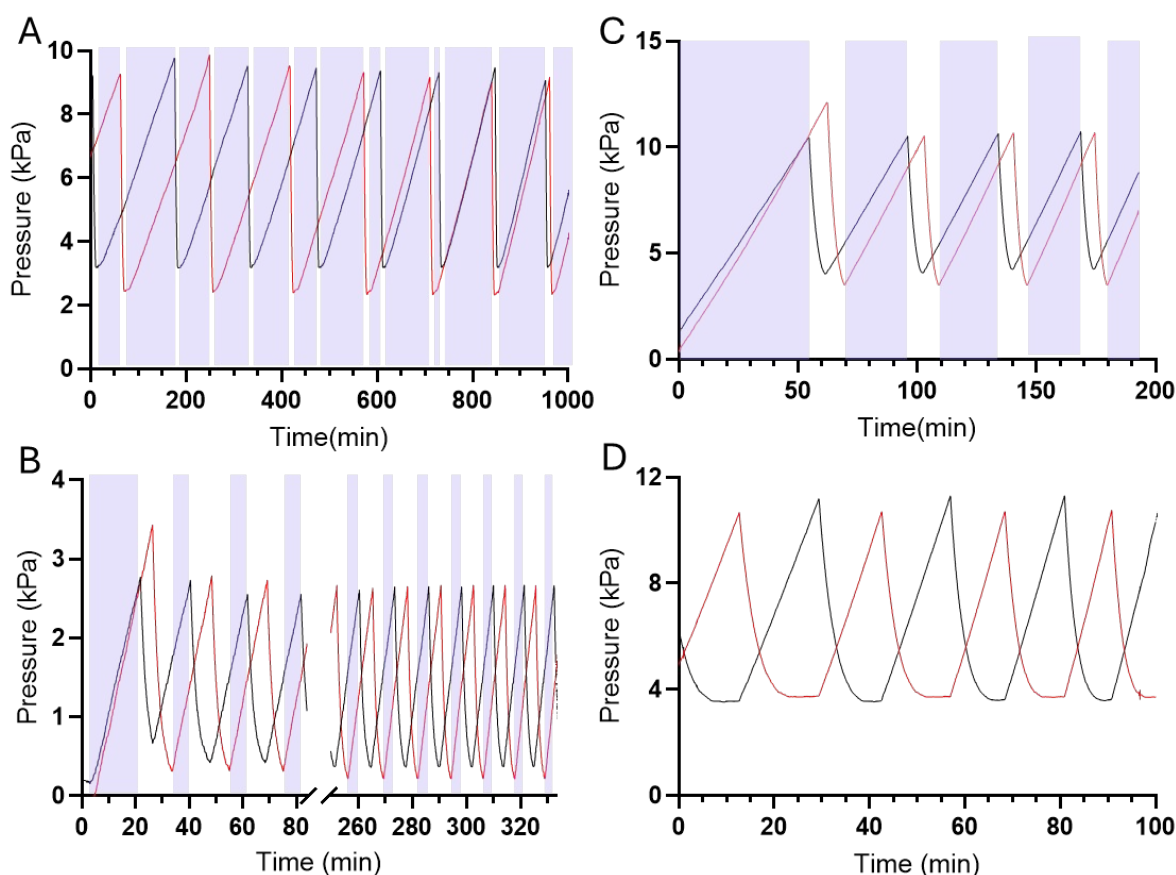
Fig. 6: Forced-air oscillator demonstrates a tri-stable oscillation at low flow rates, oscillating between an on state for 1 fluid line (valve 1 open), on-state for fluid line 2 (valve 2 open), and an off-state, where both valves are closed. In a tri-stable oscillation there are gaps between the on-states, represented in the above images by the purple block on the graphs. Tri-stable oscillations were observed in a (A) 20 \mu\text{m} thick membrane device run at 50 \mu\text{L}/\text{min} (with 60 mL syringes), (B) 20 \mu\text{m} thick membrane device run at 100 \mu\text{L}/\text{min} (with 60 mL syringes), (C) 100 \mu\text{m} thick membrane device run at 200 \mu\text{L}/\text{min} (with 140 mL syringes). There were no tri-stable oscillations in a (D) 100 \mu\text{m} thick membrane device run at 500 \mu\text{L}/\text{min} (with 140 mL syringes) and cycling only between two on-states which is indicated with no purple block.
