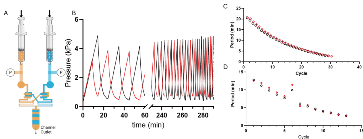
Fig. 4: Forced-air oscillators have decreasing periods over time as the syringes' fluid volumes reduce and the syringe pump continues to run. Even though the oscillation period decreases, the oscillatory behavior is persistent. A) A representative schematic of a microfluidic oscillator being driven by gas packets. Two pressure sensors, the circles with (P), upstream of the microfluidic oscillator record the pressure profiles of each fluid line. B) A 20 \mu\text{m} membrane oscillator system being driven by two 60mL syringes at a 200 \mu\text{L}/\text{min} flow rate. Graphed pressure data is split to demonstrate the stark difference in period over the first 2500 seconds compared to the (approximately) final 2500 seconds at the end of the run. C) Period decreases with each oscillation cycle for the 20 \mu\text{m} membrane oscillator and D) a 100 \mu\text{m} membrane oscillator, which was run at 500 \mu\text{L}/\text{min} .
