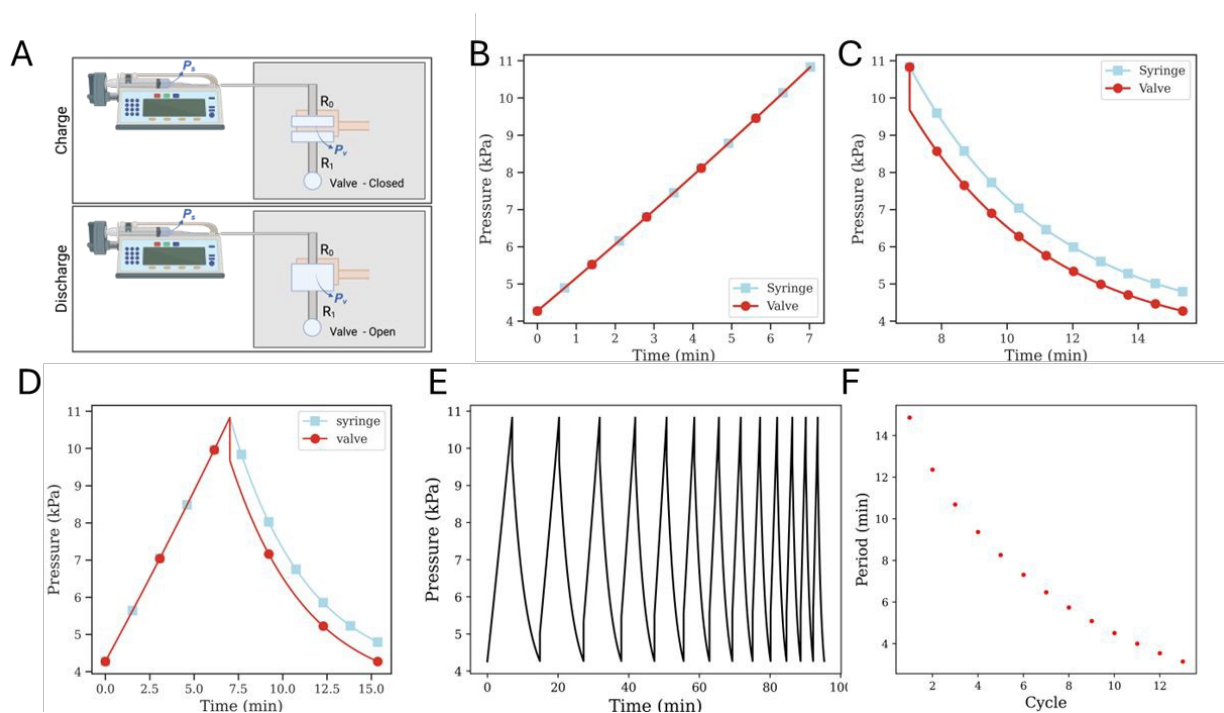
Fig. 3: (A) Oscillator full circuit schematic (B) Single pressurization cycle (C) Single depressurization cycle (D) One pressurization - depressurization cycle (E) Pressure trace for one of the valves in the oscillator system over 13 pressurization-depressurization cycles (F) Time period over 13 oscillations
