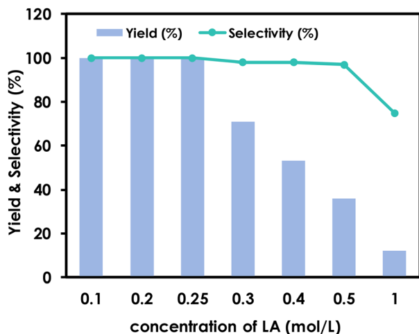
Fig. 3 Effects of LA concentration for decarboxylative protonation of LA. Reaction conditions: 0.5 mmol LA, 0.05 mmol 9-mesityl-2,7-di- tert -butyl-10-acridine (A5) (10 mol%), 0.025 mmol 4-Cl-PhSH (5 mol%), x mL DCM (0.25 M), 400 nm LEDs (20 W), Ar, room temperature (RT), 20 h. Yield and selectivity were determined by GC with n -dodecane as the internal standard.
