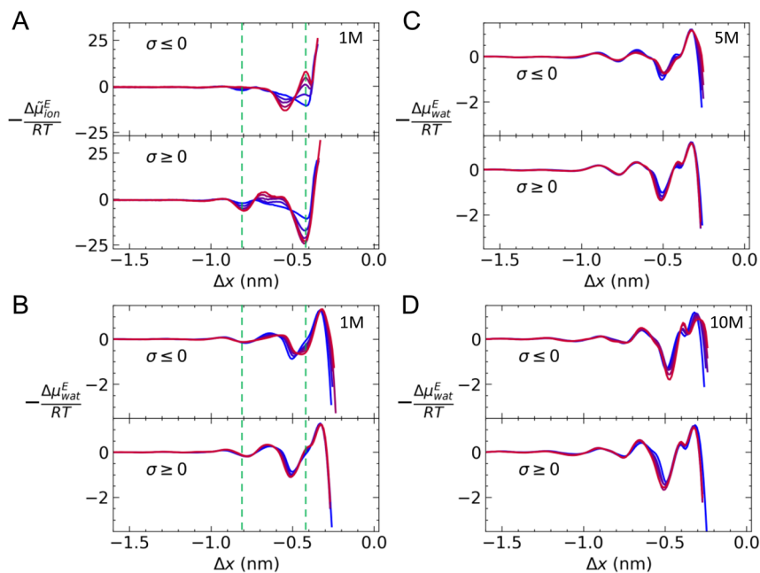
Fig. 6 (A) The excess ion electrochemical potential -\Delta\mu_{ion}^E/RT = 2 \ln(\gamma_{ion}) in solution (1 M) as a function of distance from the graphite basal surface ( \Delta x ). (B–D) The excess water chemical potential -\Delta\mu_{wat}^E/RT = \ln(\gamma(x)/\gamma^b) for water molecules as a function of \Delta x when the target bulk solution concentration was 1, 5 and 10 M, respectively. In all plots, the top and bottom panels provide data for solutions at negatively and positively charged surfaces, respectively; blue \rightarrow red colours indicate |\sigma| = 0 \rightarrow 0.77 e \text{ nm}^{-2} . Green dashed lines highlight the position of the first two minima in -\Delta\mu_{ion}^E/RT when \sigma = 0 .
