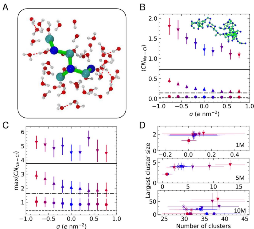
Fig. 3 (A) A [Na_3Cl_4]^- cluster at the carbon surface surrounded by its solvation sphere. Na^+ , Cl^- , O and H atoms are shown by blue, cyan, red and white spheres, respectively. Green lines highlight ion connections within 0.4 nm, and H-bonds are indicated by the red dashed lines. (B) Average Na–Cl coordination number ( \langle CN_{Na-Cl} \rangle ) in the EDL as a function of surface charge density, \sigma . (C) Average maximum ( max ) CN_{Na-Cl} in the EDL. In B and C, \circ , \Delta and \nabla symbols indicate data for 1, 5 and 10 M with dashed, dotted-dashed and solid lines highlighting the bulk values at 1, 5 and 10 M. (D) Number of clusters and largest cluster size in the EDL at the positive ( \times ) and negative electrode ( \nabla ) with the bulk ( \circ ) values also provided.
