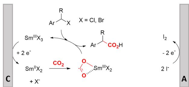
Fig. 4 Mechanism of the carboxylation of benzylic halides using a Sm(II)/Sm(III) catalyst. C = cathode, A = anode. Adapted from ref. 138.
