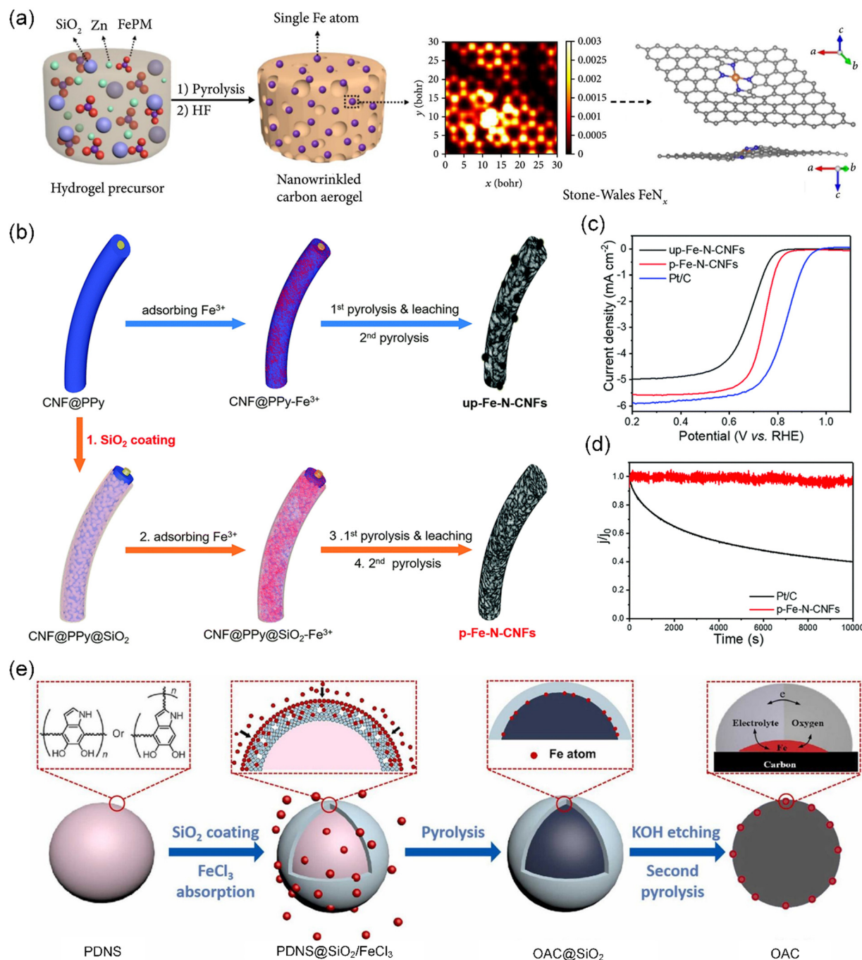
Fig. 3 \text{SiO}_2 -assisted carbonization strategy. (a) Schematic representation of the synthesis of the \text{NCA}_{C-zn}/\text{Fe} carbon aerogel. Reproduced with permission from ref. 80 (Copyright 2019, AAAS). (b) Schematic illustration of the fabrication of up-Fe-N-CNF (top) and p-Fe-N-CNF (bottom) catalysts. (c) Linear sweep voltammetry (LSV) curve of up-Fe-N-CNFs, p-Fe-N-CNFs, and Pt/C. (d) Chronoamperometric test of p-Fe-N-CNFs and Pt/C at 0.45 V vs. RHE. (b)–(d) Reproduced with permission from ref. 81 (Copyright 2018, The Royal Society of Chemistry). (e) Schematic illustration of the preparation of CNS with single Fe atoms at the triple-phase boundary. Reproduced with permission from ref. 82 (Copyright 2022, ScienceDirect).
