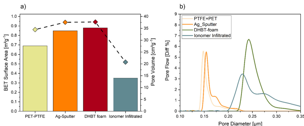
Fig. 7 Characterization of the microstructure at each processing step during GDE manufacturing. (a) Calculated BET surface area by and measured pore volume by capillary flow porosimetry, (b) distribution of pore diameters.
