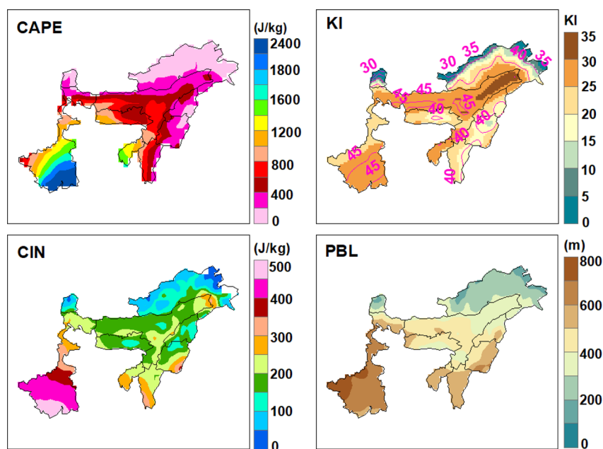
Fig. 3 Climatological convective available potential energy (CAPE), K -index (KI), convective inhibition (CIN) and planetary boundary layer (PBL) during pre-monsoon derived from ERA5 for the period 1980–2020. Contours in pink colour in the top (right panel for KI) represent the total totals index (TTI) values for the same period.
