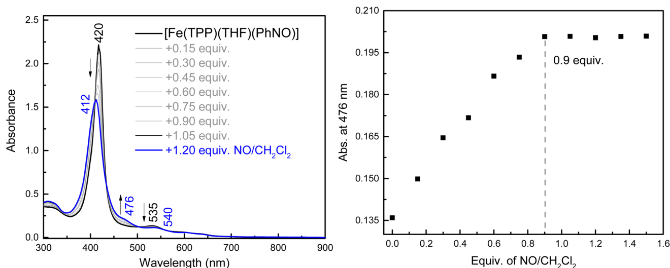
Fig. 8 UV-Vis spectra of the titration of \sim 14 \mu\text{M} [\text{Fe}(\text{TPP})(\text{THF})(\text{PhNO})] (black) in THF with a NO-saturated solution of dichloromethane, forming the ferrous NO complex [\text{Fe}(\text{TPP})(\text{NO})] (blue). Right: Changes in absorbance at 476 nm upon addition of the NO solution, showing that the reaction is complete after the addition of \sim 1 equivalent of the NO-saturated dichloromethane solution.
