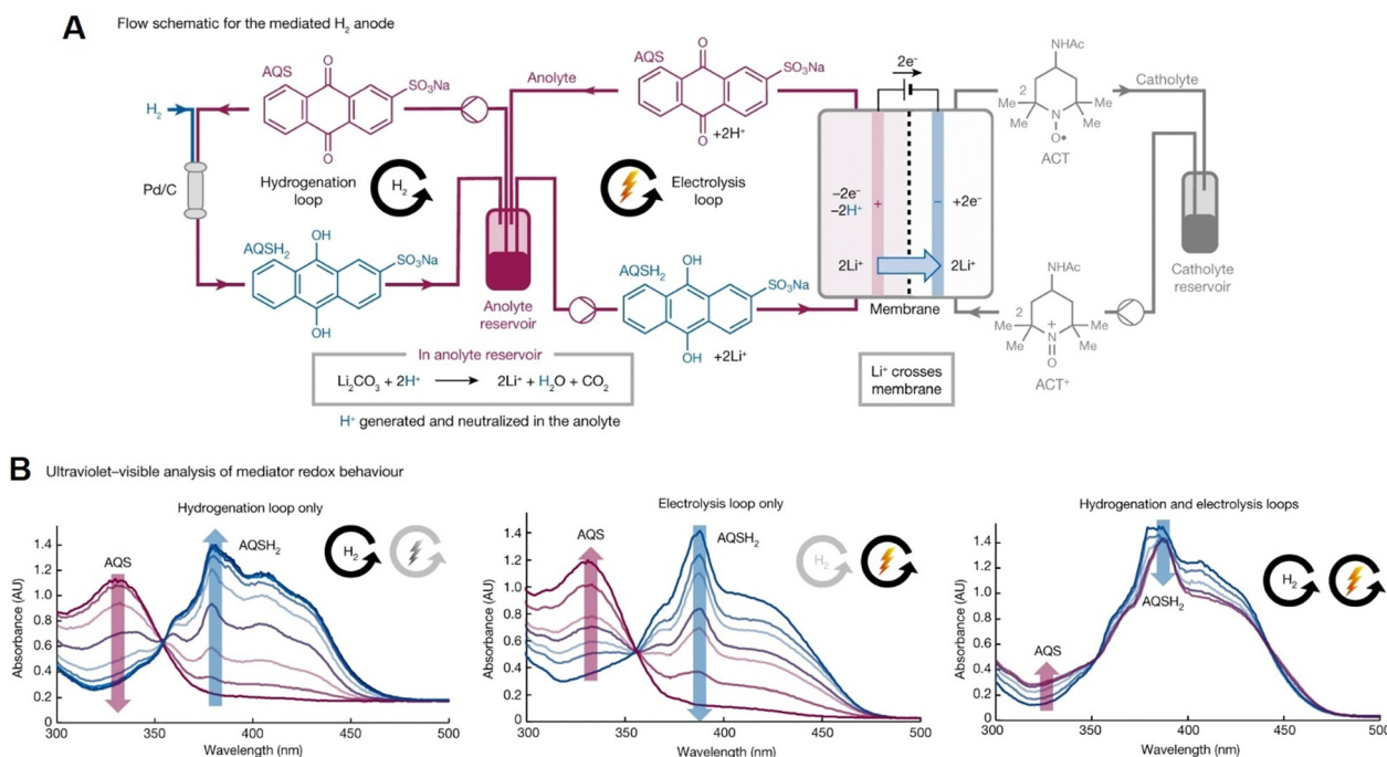
Fig. 18 (A) Schematic of mediated \text{H}_2 anode by pairing the thermal hydrogenation of AQS and the electrochemical oxidation of \text{AQS} + 2\text{H}^+ in real time. (B) In situ UV-Vis spectra of the redox speciation of AQS and \text{AQS} + 2\text{H}^+ species in the anolyte reservoir for various processes, such as hydrogenation-only or electrolysis-only loop, or both loops operating simultaneously. Reproduced with permission from ref. 215. Copyright 2023 Springer Nature.
