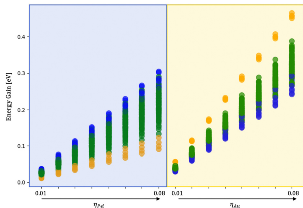
Fig. 8 Energy gain per atom for AuPd in various environments w.r.t. the vacuum varying the strength of Pd (blue shadow)/Au (yellow shadow) interaction ( \eta_x ), fixing \rho_x at 1.5. Orange circles represent core-shell initial configurations, mixing configurations are in blue and Janus-like in green. An inversion of the chemical ordering stability occurs as soon as only Pd interacts while AuPd favours core (Pd)-shell (Au) ordering.
