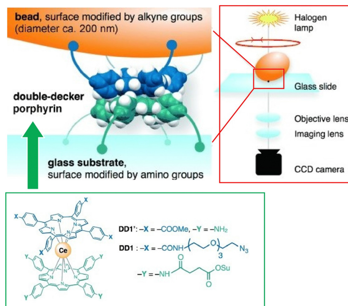
Fig. 12 Single-molecule imaging and manipulation using optical microscopy for evaluation of a synthetic molecular rotor, a double-decker porphyrin with magnetic bead. Reprinted with permission from ref. 76. Copyright 2014 Wiley-VCH.
