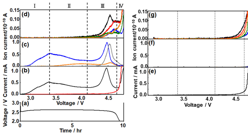
Fig. 3 (a) Discharge curve of a Li/TEGDME-1M LiTFSI/KJCNT cell (electrode area: 2 \text{ cm}^2 ) obtained under a constant current of 0.4 \text{ mA} ( 0.2 \text{ mA cm}^{-2} ). (b and e) Current, (c and f) signal intensities of m/z = 18 ( \text{H}_2\text{O}^+ ): orange, m/z = 32 ( \text{O}_2^+ ): blue, and m/z = 44 ( \text{CO}_2^+ ): gray (middle panel), and (d and g) intensities of mass signals of fragments related to organic molecules derived from TEGDME, i.e. , m/z = 28 ( \text{CO}^+ ): black, m/z = 29 ( \text{COH}^+ ): red, m/z = 30 ( \text{HCOH}^+ ): blue, m/z = 31 ( \text{CH}_3\text{OH}^+ , \text{CH}_2\text{OH}^+ ): green, and m/z = 45 ( \text{CH}_3\text{OCH}_2^+ , \text{COOH}^+ ): orange, as a function of cell voltage during the potential sweep with 0.05 \text{ mV s}^{-1} after (b–d) and without discharge (e–g). The current response without discharge (e) is also shown in (b) (red line) for a comparison. Note: the scales for the y -axis of (c and f) are 8 times larger than those of (d and g).
