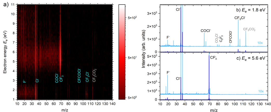
Fig. 5 (a) 2D mass spectra of negative ions produced by electron attachment to \text{CF}_3\text{COCl} molecules at different electron energies. (b) and (c) Mass spectra at two different electron energies.
