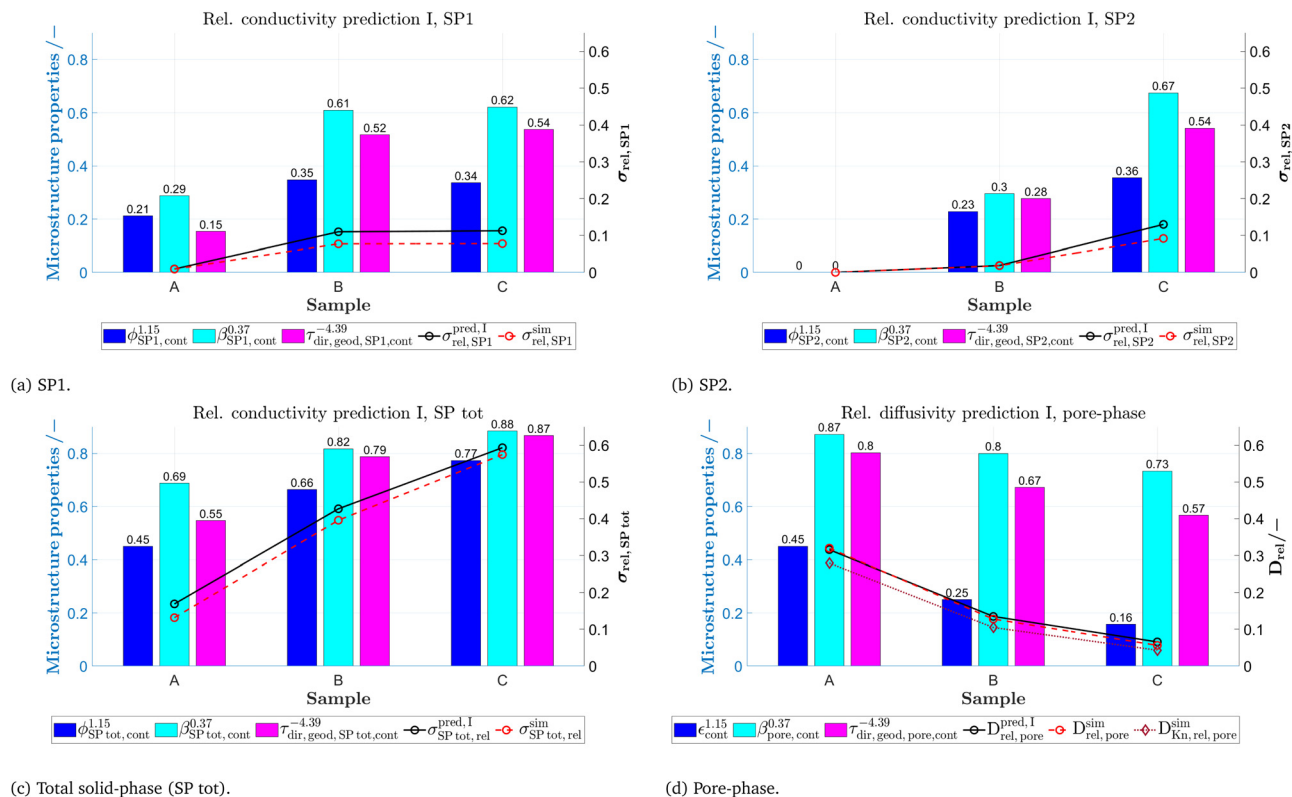
Fig. 24 M -factor prediction I (black lines) and its three components (volume fraction effect \phi^{1.15} , constricitivity effect \beta^{0.37} and tortuosity effect \tau_{dir,geod}^{-4.39} ) and simulated M -factors (red lines), for (a) SP1, (b) SP2, (c) total solid-phase (SP tot) and (d) the pore-phase of the sphere-packing structures. The used variables are summarized in the Tables 9 and 10.
