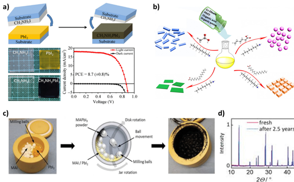
Fig. 14 (a) Schematic illustration of the fabrication process of perovskite films using a solid-state reaction (top) and the corresponding photographs of the real films (bottom-left). The J - V curves of the perovskite solar cells prepared using the solid-state chemical reaction method under AM 1.5G irradiation and in the dark (bottom-right). Adapted with permission from ref. 210. (b) Schematic illustrating the formation processes for different \text{CsPbX}_3 (where X = \text{Cl}, \text{Br}, \text{I} ) nanocrystals mediated by organic acid and amine ligands at room temperature: hexanoic acid and octylamine for spherical quantum dots; oleic acid and dodecylamine for nanocubes; acetate acid and dodecylamine for nanorods; and oleic acid and octylamine for few-unit-cell-thick nanoplates. Adapted with permission from ref. 222. (c) Photograph of a milling jar loaded with milling balls, MAI, and \text{PbI}_2 precursor powders (left), schematic of the ball milling procedure for the mechanochemical synthesis of perovskite powders (middle), and photograph of the milling jar after the ball milling process and successful mechanochemical synthesis of black \text{MAPbI}_3 powder (right). (d) XRD patterns of \text{MAPbI}_3 powders before and after more than two and a half years of storage in a dry atmosphere. Adapted with permission from ref. 237.
