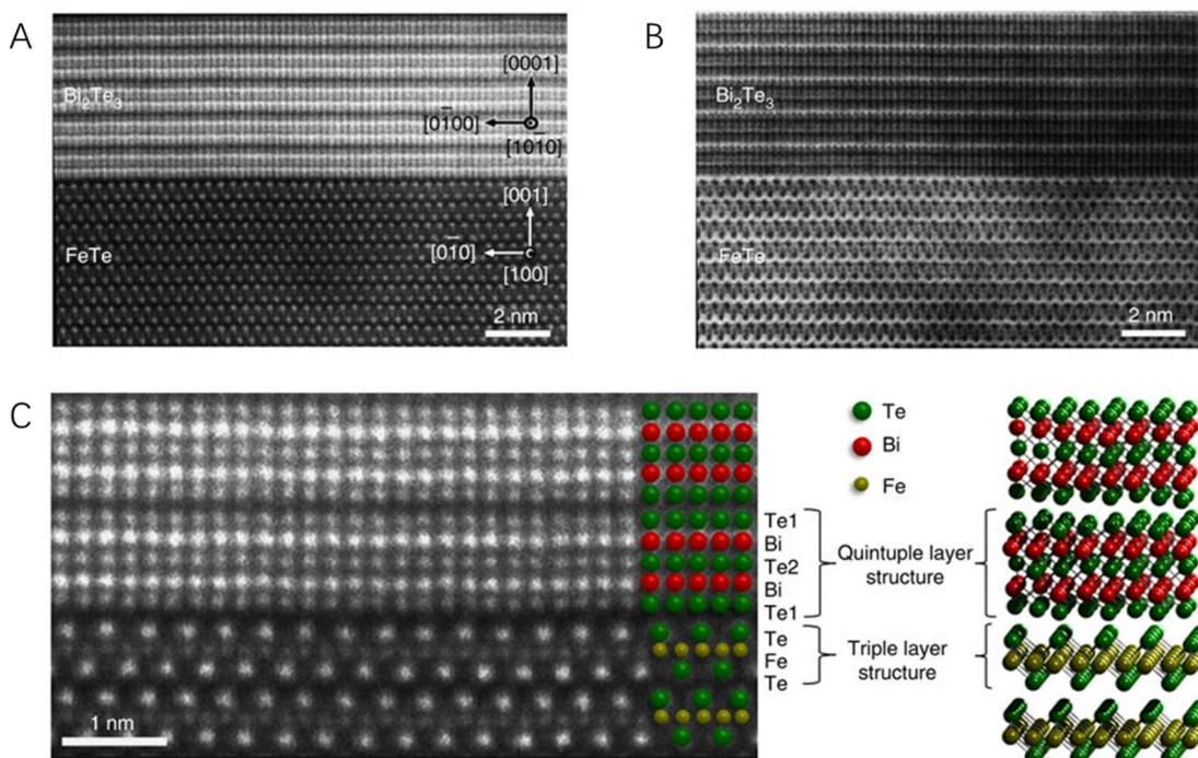
Fig. 5 The scanning transmission electron microscopy micrographs of a \text{Bi}_2\text{Te}_3/\text{FeTe} heterostructure. (A) The HAADF image. (B) The annular bright field image. (C) The higher-magnification HAADF image showing the atomically sharp interface between \text{Bi}_2\text{Te}_3 and FeTe. Reproduced with permission from ref. 75, copyright Springer Nature.
