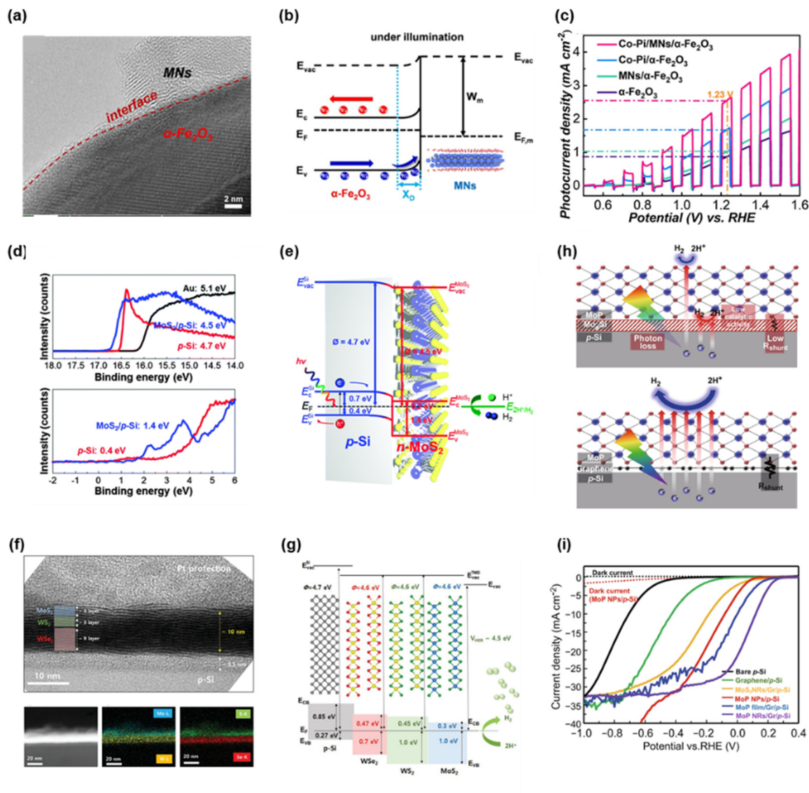
Fig. 3 (a) High-resolution TEM image of MXene nanosheets/ \alpha - \text{Fe}_2\text{O}_3 . (b) Energy band diagram of MXene nanosheets/ \alpha - \text{Fe}_2\text{O}_3 Schottky junction under illumination. (c) LSV curves of \alpha - \text{Fe}_2\text{O}_3 , MNs/ \alpha - \text{Fe}_2\text{O}_3 , Co-Pi/ \alpha - \text{Fe}_2\text{O}_3 , and Co-Pi/MNs/ \alpha - \text{Fe}_2\text{O}_3 . Copyright 2021, Elsevier. (d) UPS and XPS spectra of Au, p-Si, and \text{MoS}_2/\text{p-Si} . (e) Schematic of energy band diagram of the \text{MoS}_2/\text{p-Si} photocathode having p-n junction. Copyright 2016, Royal Society of Chemistry. (f) Cross-sectional high-resolution TEM image for 112-MWW/ \text{p-Si} thin film. Copyright 2019, Wiley-VCH GmbH. (g) Schematic of energy band diagram of 112-MWW/ \text{p-Si} thin film. Copyright 2019, Wiley-VCH GmbH. (h) Schematic of MoP/ \text{Mo}_3\text{Si}/\text{p-Si} and MoP/graphene/ \text{p-Si} . (i) LSV curves of bare p-Si, graphene/p-Si, \text{MoS}_2 NRs/Gr/p-Si, MoP NPs/p-Si, MoP film/Gr/p-Si, and MoP NRs/Gr/p-Si. Copyright 2021, Springer Nature.
