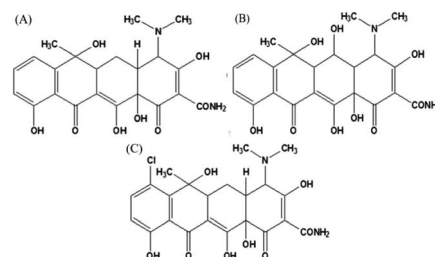
Fig. 1 Chemical structure of (A) tetracycline, (B) oxytetracycline, and (C) chlortetracycline.
