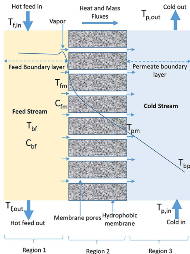
Fig. 4 Temperature polarization phenomenon in MD. T_{f,in} , T_{f,m} , T_{p,m} and T_{p,b} represent temperatures in the bulk feed solution, near the membrane surface (feed side), near the membrane surface (permeate side) and in the bulk permeate, respectively. 58
