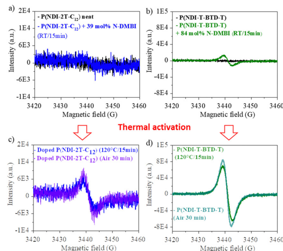
Fig. 5 EPR spectra of (a) neat P(NDI-2T-C12) and P(NDI-2T-C12):N-DMBI mixed at RT in toluene (inert atmosphere, in dark). (b) Neat P(NDI-T-BTD-T) and P(NDI-T-BTD-T):N-DMBI mixed at RT in chlorobenzene (inert atmosphere, dark). (c) and (d) Same solutions heated up at 120 °C in inert atmosphere and exposed to air. Magnetic field power: 158.63 mW, modulation amplitude: 3.0 G.
