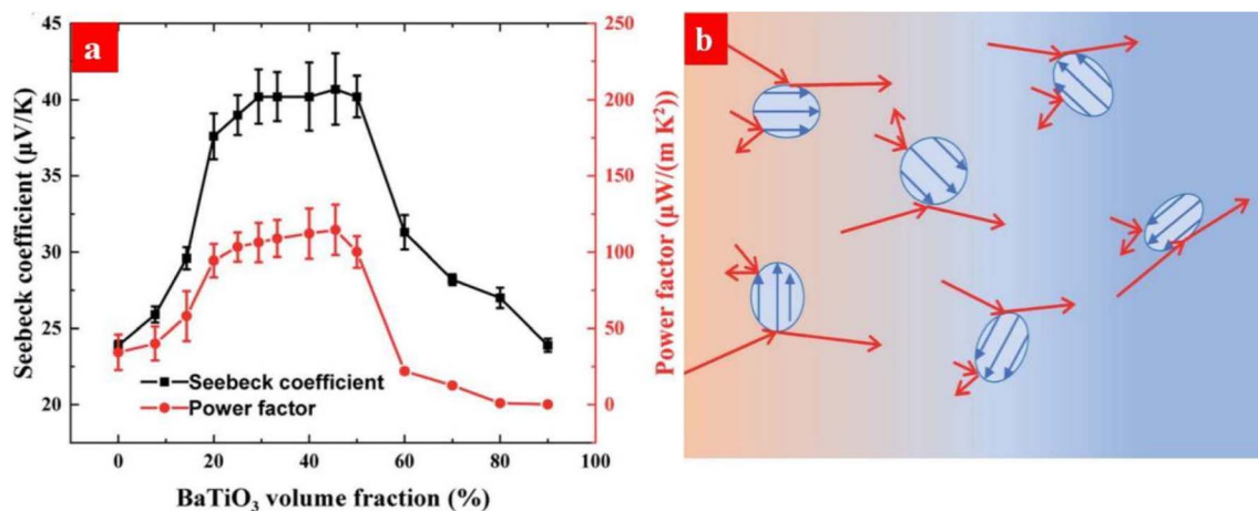
Fig. 15 (a) Changes of the Seebeck coefficient and power factor of PEDOT:PSS/BaTiO 3 films. (b) Schematic diagram of energy filtering of PEDOT:PSS by the ferroelectric BaTiO 3 nanoparticles (blue dots). The blue and red arrows are for the spontaneous electric polarization in the BaTiO 3 nanoparticles and the hole transport, respectively. The charge carriers migrate from the hot end (red regions) to the cold end (blue regions) under a temperature gradient. Reproduced with permission. 178 Copyright 2021, Royal Society of Chemistry.
