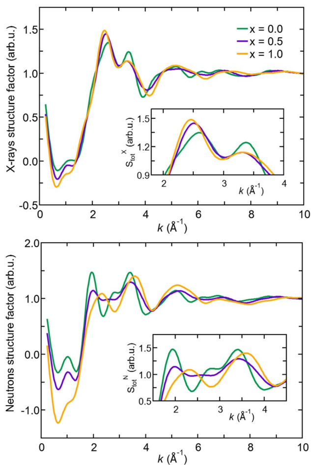
Fig. 2 (Color online) Total X-ray (top) and neutron (bottom) structure factors for amorphous Na_{3-x}OH_xCl ( x = 0, x = 0.5 , and x = 1 ) obtained through Fourier transform of the total pair correlation functions at T = 300 \text{ K} . Insets: zoomed-in view of the 1.8\text{--}4.0 \text{ \AA}^{-1} and 1.5\text{--}4.5 \text{ \AA}^{-1} ranges, respectively.
