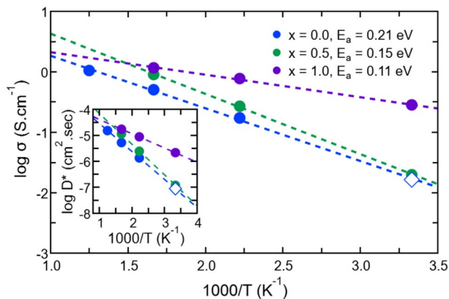
Fig. 12 (Color online) Na-ion self-diffusion coefficients (inset) and conductivities of amorphous \text{Na}_{3-x}\text{OH}_x\text{Cl} ( x = 0, x = 0.5 , and x = 1 ). We also report the activation energies of Na ionic conduction obtained via a linear Arrhenius fit. Closed circles correspond to FPMD data and open circles correspond to data at T = 300 K extrapolated by using the linear Arrhenius fit.
