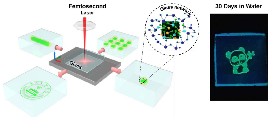
Fig. 9 Scheme of the 3D perovskite patterns generated inside the glass matrix by using femtosecond laser irradiation and the digital image of CsPbBr 3 patterns after being stored in water for 30 days (modified with permission from ref. 41).
