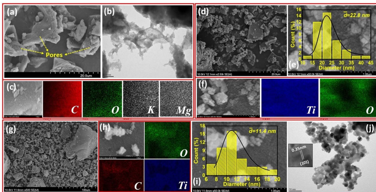
Fig. 1 (a) SEM image, (b) TEM image, and (c) EDS maps of spent-coffee ground biochar (CGB); (d) SEM image, (e) particle size distribution and (f) EDS maps of TiO 2 ; and (g) SEM image, (h) EDS mapping, (i) particle size distribution and (j) TEM image of CGBT nanocomposites.
