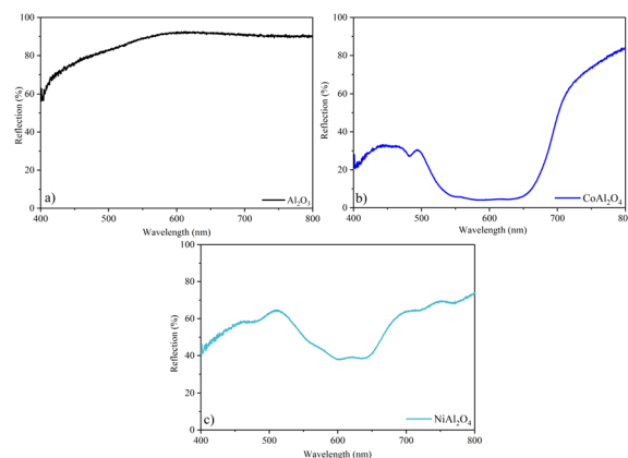
Fig. 12 Reflection spectra in the visible region: (a) Al 2 O 3 (alumina), (b) CoAl 2 O 4 (cobalt aluminate), and (c) NiAl 2 O 4 (nickel aluminate).
