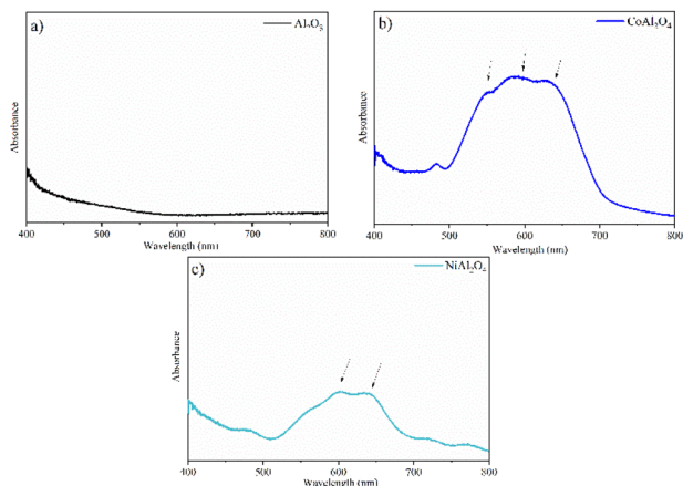
Fig. 8 Absorption spectra in the visible region: (a) Al 2 O 3 (alumina), (b) CoAl 2 O 4 (cobalt aluminate) and (c) NiAl 2 O 4 (nickel aluminate).
