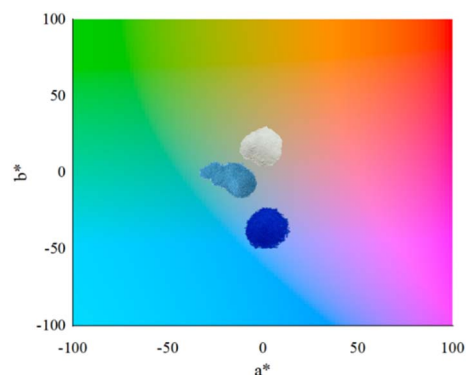
Fig. 10 Al 2 O 3 (alumina), CoAl 2 O 4 (cobalt aluminate), and NiAl 2 O 4 (nickel aluminates) distribution according to color quadrant.
