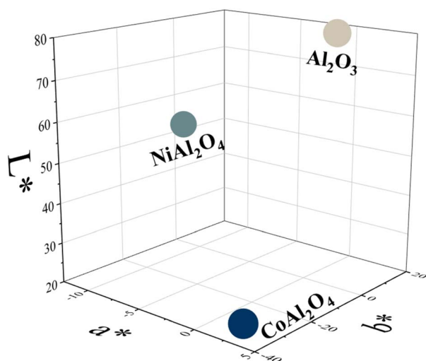
Fig. 9 Distribution of Al 2 O 3 (alumina), CoAl 2 O 4 (cobalt aluminate), and NiAl 2 O 4 (nickel aluminate) in 3D CIE L*a*b* color space.
