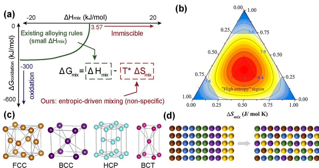
Fig. 1 (a) Enabling more alloy choices based on the entropic contribution ( -\Delta S_{\text{mix}} ). Reproduced with permission. 32 Copyright 2021, Elsevier Ltd. (b) Different spaces of traditional alloy and high entropy alloy. Reproduced with permission. 33 Copyright 2016, Elsevier Ltd. (c) HEAs structure model. Reproduced with permission. 32 Copyright 2021, Elsevier Ltd. (d) High entropy effect.
