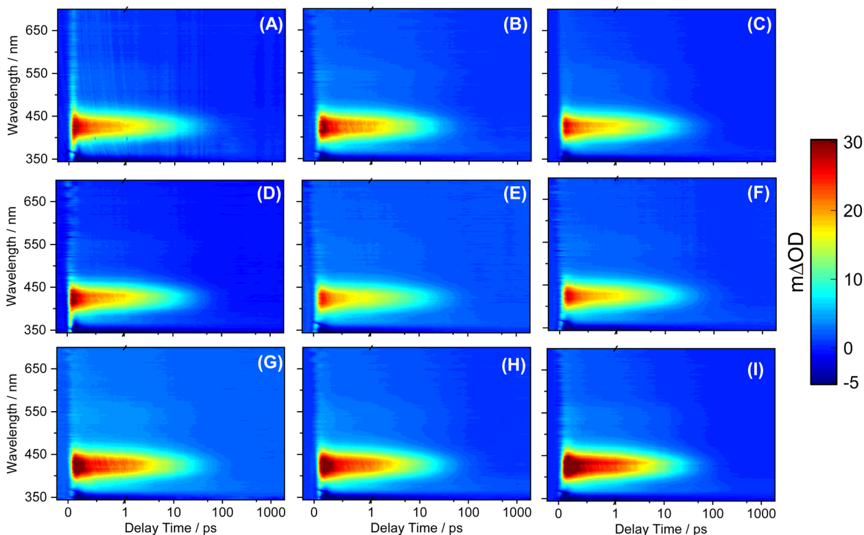
Fig. 4 TEA spectra in caprylic capric triglyceride bulk solution for (A) SM, (B) DESM, (C) DBSM (D) DOSM, (E) DLSM, (F) DCSM, (G) DGSM, (H) DFSM, and (I) DOleySM in the form of a false colour heat map indicating change in optical density ( \Delta OD ). In all cases, the delay time is presented on a linear plot until 1 ps and then as a logarithmic scale between 1 ps and 2 ns.
