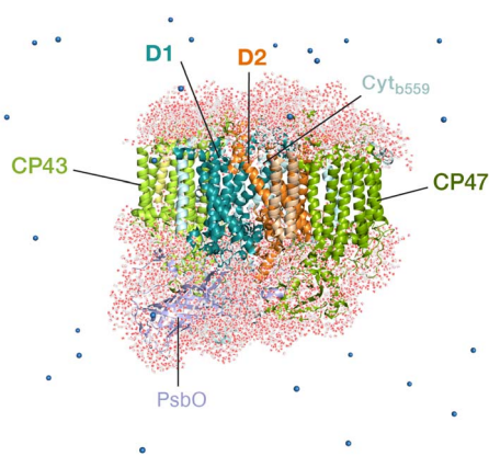
Fig. 2 The all-atom model of the PSII monomer used for the QM/MM computations, indicating selected major protein subunits. Appropriate number of sodium ions were retained to maintain charge neutrality of the model. The overall system contains 76 056 atoms.
