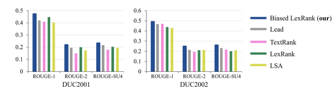
Fig. 9 The performance of the proposed method is compared with the baseline in terms of multiple metrics on DUC2001 and DUC2002.
