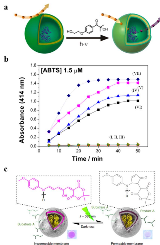
Fig. 6 (a) Schematic representation of UV-responsive nanoreactors. (b) HRP activity test. (I–III) HRP-filled polymersomes before photoreaction with 2-hydroxy-4'-2-(hydroxyethoxy)-2-methyl-propiophenone (PP-OH) and (IV–VII) after photoreaction with PP-OH. (IV) A-PMOXA- b -PDMS- b -PMOXA-A-HRP-PP-OH. (V) PMOXA- b -PDMS- b -PMOXA-HRP-PP-OH. (VI) PEO- b -PB-HRP-PP-OH. (VII) Free HRP. Reprinted from ref. 88. Copyright 2013, American Chemical Society. (c) The catalytic activity of the DASA esterase nanoreactor is activated by green light irradiation and deactivated by fading light irradiation. Reprinted from ref. 89. Copyright 2023, Springer Nature.
