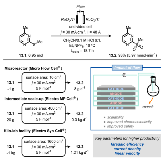
Fig. 13 Adoption of flow electrochemistry in an industrial context for the highly scalable, selective anodic oxidation of thioether 13.1 . t_{\text{reirc.}} : time of recirculation.
