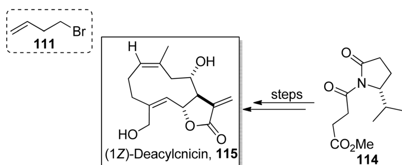
Scheme 12 Total synthesis of (1Z)-deacylnicin 115.
