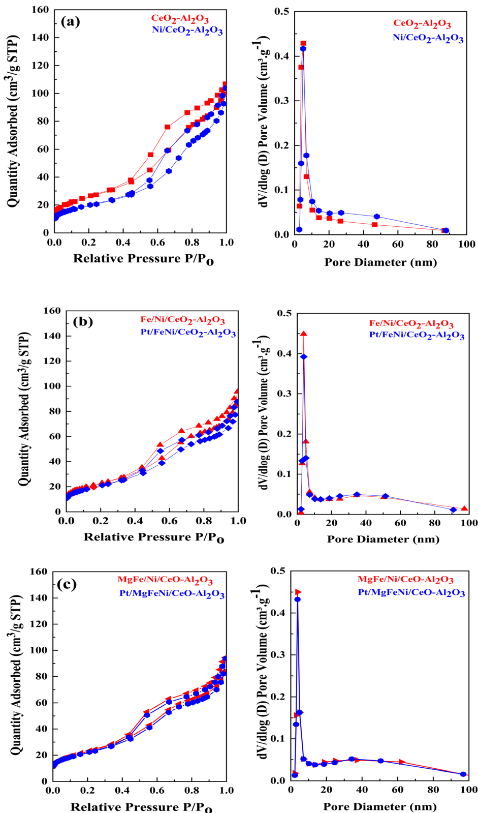
Fig. 5 ((a–c), left side) \text{N}_2 physisorption isotherms and ((a–c), right side) BJH pore size distribution of of Ni-based \text{Al}_2\text{O}_3 - \text{CeO}_2 composite catalysts.
