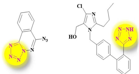
6-azidotetrazolo[5,1-a]phthalazine Losartan
