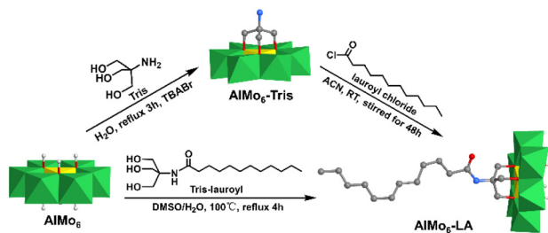
Fig. 8 Synthesis of AlMo 6 -LA by pre- or post-modification methods. Color code: {MoO 6 }, green octahedron; {AlO 6 }, yellow octahedron; Cl, gray; O, deep red; N, light blue; H, light grey.
