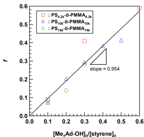
Fig. 4 Linear dependence of the f value on the initial ratio of Me 2 Ad-OH to the styrene unit.
