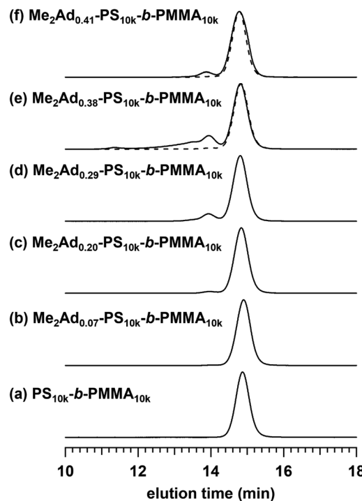
Fig. 5 SEC traces of Me 2 Ad-PS 10k - b -PMMA 10k samples (b)-(f) and the corresponding PS 10k - b -PMMA 10k (a) (eluent, THF; flow rate, 1.0 mL min -1 ). The dashed curves represent the SEC traces after preparative SEC purification.
