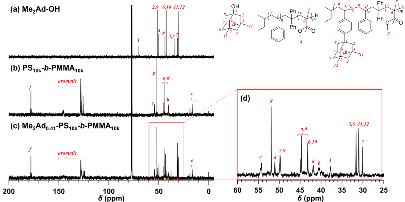
Fig. 3 13 C NMR spectra of (a) Me 2 Ad-OH and (b) PS 10k - b -PMMA 10k in CDCl 3 (100 MHz), and (c) inverse-gated decoupling 13 C NMR spectrum of Me 2 Ad 0.41 -PS 10k - b -PMMA 10k (lower) in CDCl 3 (100 MHz). (d) The expansion from 60 to 25 ppm of the spectrum (c).
