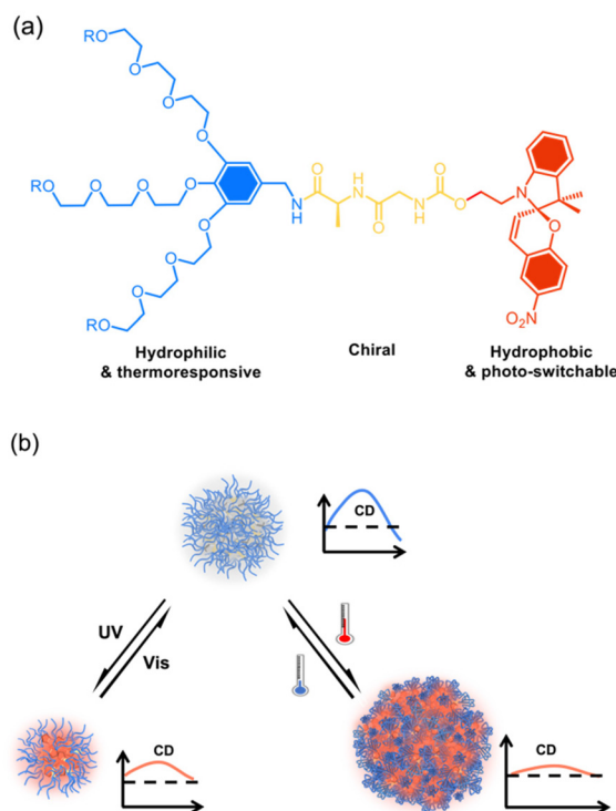
Chart 1 Illustration of supramolecular assembly of the dendronized spiropyrans (DSPs) (a) in aqueous solutions into chiral spheres with chiralities dually tunable by irradiation and temperature (b).
