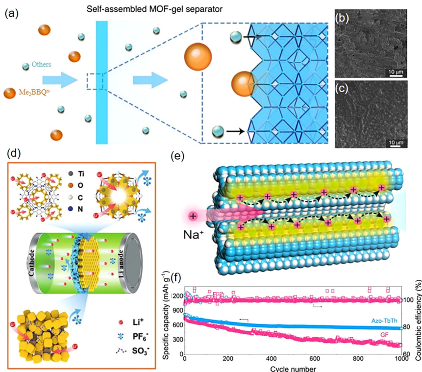
Fig. 24 (a) Schematic illustration of MOF-gel separator for limiting \text{Me}_2\text{BBQ}^- . Comparison of SEM images of the deposition morphology of lithium metal electrodes using a common separator (b) and MOF-gel separator (c). Reproduced with permission. 216 Copyright 2020, Springer Nature. (d) Schematic diagram of MOFs@PP separator regulating \text{Li}^+ and anion migration in LMBs. Reproduced with permission. 217 Copyright 2021, Wiley-VCH GmbH. (e) Schematic profile of \text{Na}^+ rapid migration mechanism in Azo-TbTh separator. (f) Cyclic stability of Na-S batteries assembled with Azo-TbTh and GF as separators at 1 C. Reproduced with permission. 220 Copyright 2022, the American Chemical Society.
