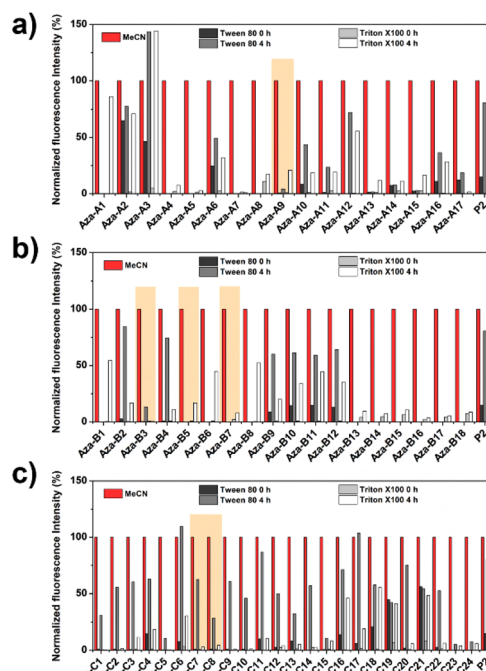
Fig. 4 Normalized fluorescence re-illumination of novel ACQ probes ( 250 \text{ nmol L}^{-1} compared with acetonitrile): (a) Type A Aza-BODIPY; (b) Type B Aza-BODIPY; (c) Type C Aza-BODIPY) in surfactant 1% Tween 80 and 1% Triton X100. The excitation was set at the wavelength blue-shifted by 20 nm compared to the maximal absorption wavelength of the probe (slit: 5/5 nm).
