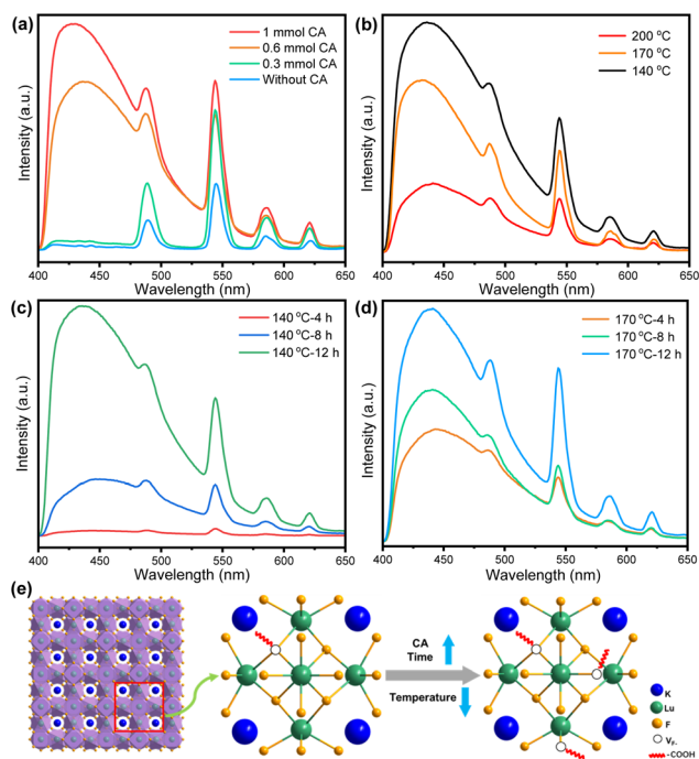
Fig. 3 PL spectra of \text{KLu}_3\text{F}_{10}:\text{15Tb} synthesized with different CA contents (a), different reaction temperatures (b), different hydrothermal reaction times at 140 ^\circ\text{C} (c) and 170 ^\circ\text{C} (d). (e) Schematic illustration of the proposed defect formation mechanism.
