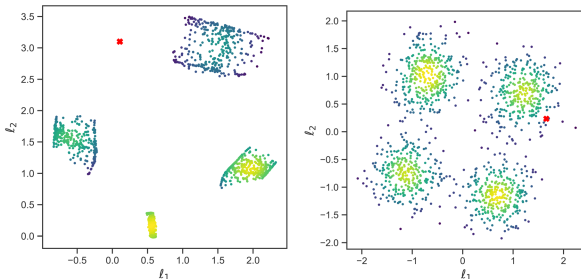
Fig. 8 Plot showing latent space representation of a traditional autoencoder (left) versus a variational autoencoder (right). Both have latent dimensionality n_l = 2 , and \ell_1 and \ell_2 are latent space variables. The VAE has Kullback–Liebler divergence \beta = 1 . Red crosses correspond to the SLD curve labeled as “Fit: ad hoc ” in Fig. 5b.
