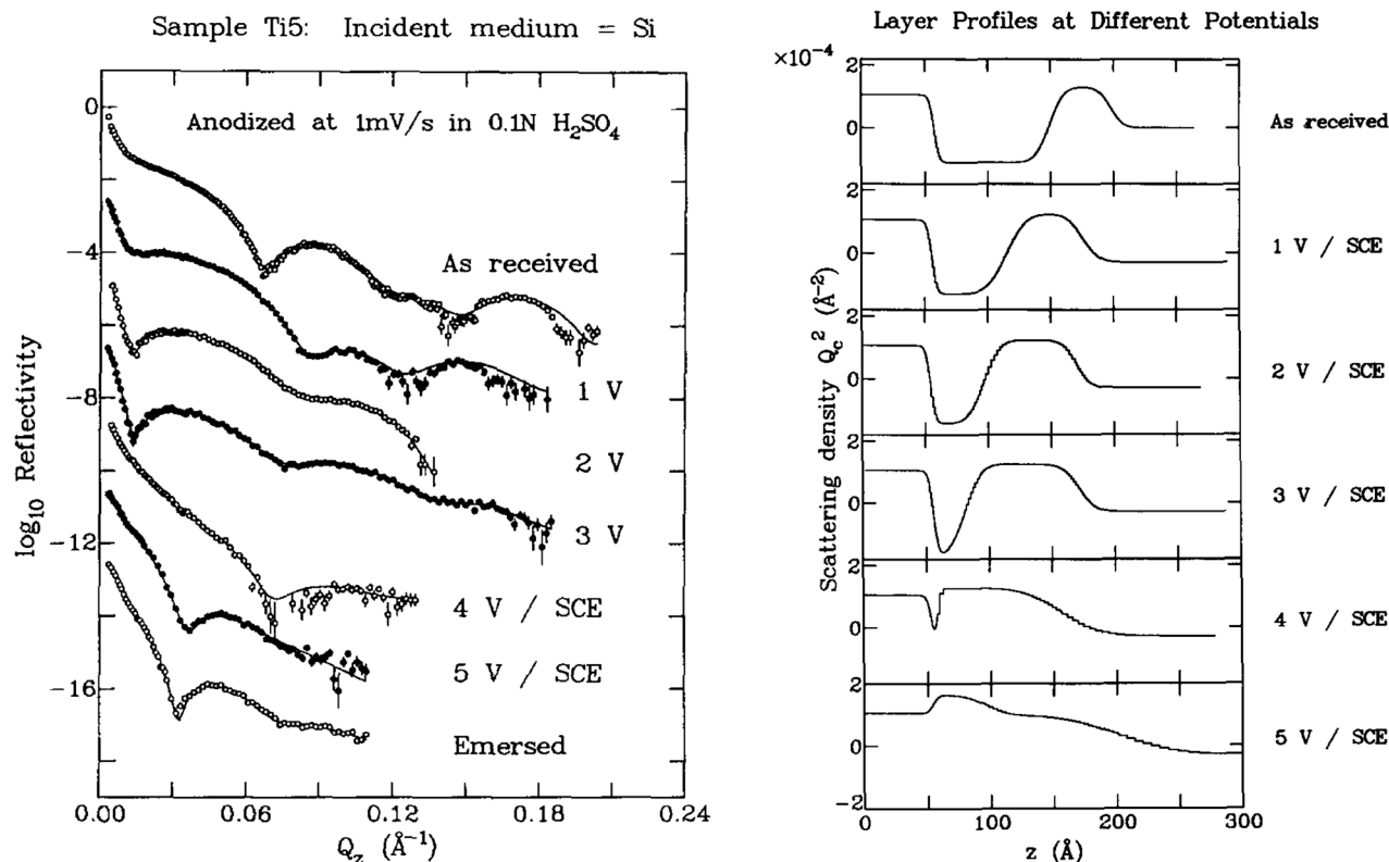
Fig. 8 On the left are shown NR data for various states of oxidation of a titanium film in contact with an electrolyte in an aqueous reservoir as originally obtained by Wiesler et al. 16 and shown in Fig. 1 of their paper. The open circles are data points whereas the solid lines represent fits of the data using the corresponding SLD profiles displayed on the right-hand side of the figure (after Fig. 2 of Wiesler et al. 16 ). In the SLD plots, the silicon substrate is on the left and the aqueous reservoir on the right (note that the SLD is characterized in terms of the critical angle or Q_c for Si as opposed to the more conventional unit of \text{\AA}^{-2} as is current practice). The data suggest a systematic growth of the TiO layer at the expense of the Ti with increasing applied voltage. (Note that the SLD for titanium metal is a negative quantity which is relatively uncommon for most isotopes.)
