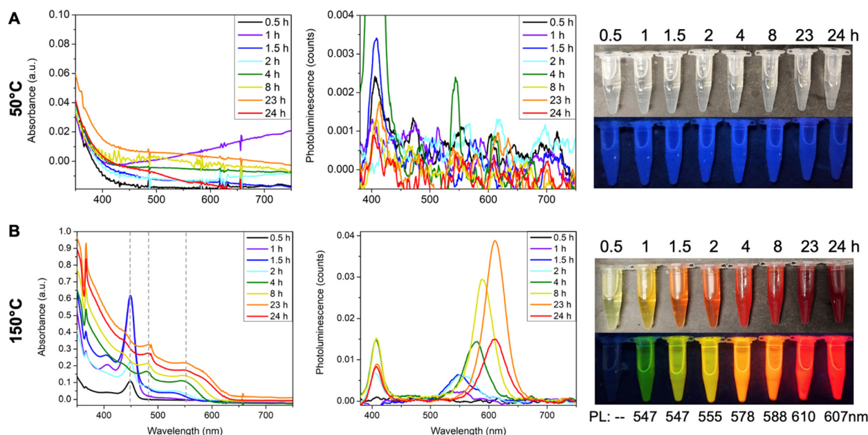
Fig. 5 Effect of temperature on CdTe MSC formation. The reactions at (A) 50 °C and (B) 150 °C are monitored by absorbance, emission, and photos of aliquots under ambient light and UV light, respectively.
