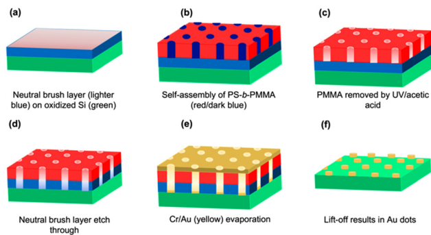
Fig. 1 (a)–(f) Schematic illustration of Au dot formation.
