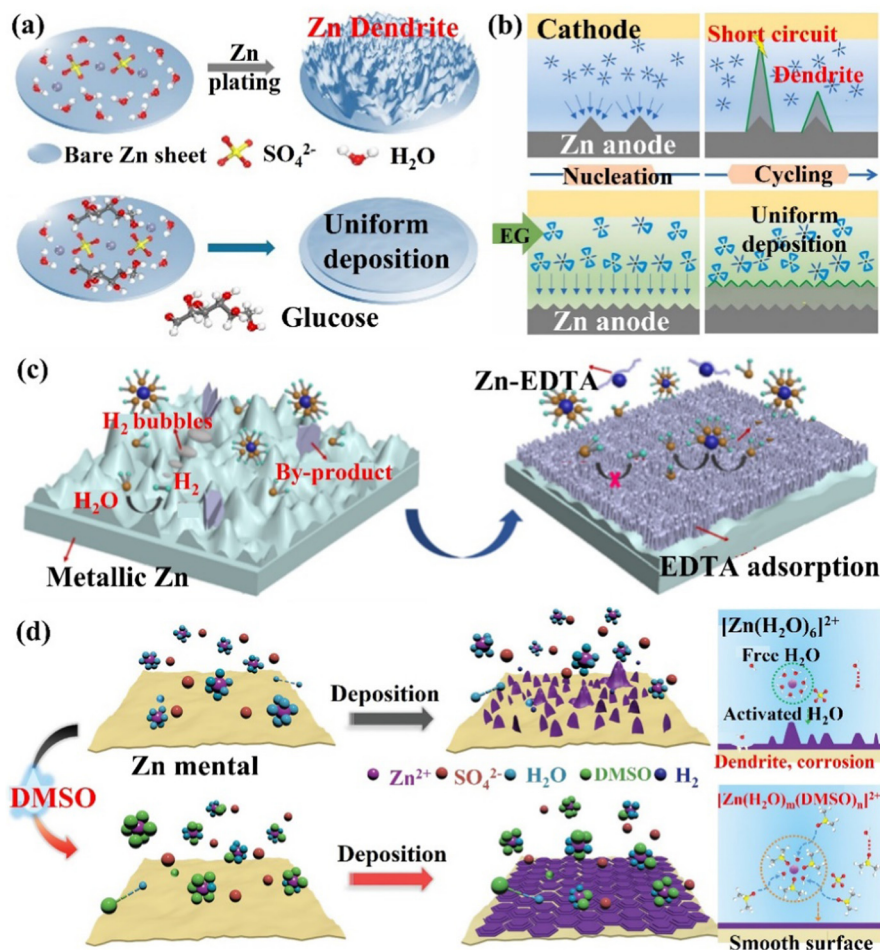
Fig. 15 The schematic diagram of (a) Zn deposition behaviors in ZnSO 4 and ZnSO 4 –glucose electrolytes. Reproduced with permission from ref. 66. Copyright 2021, Wiley-VCH. (b) A schematic diagram of dendrite inhibition of ZnSO 4 /H 2 O/EG hybrid electrolytes. Reproduced with permission from ref. 32. Copyright 2020, Elsevier Inc. (c) A schematic of Zn/electrolyte interphase behaviors during Zn plating in ZnSO 4 electrolyte and EDTA-functionalized ZnSO 4 electrolyte. Reproduced with permission from ref. 160. Copyright 2021, Wiley-VCH. (d) A diagram of the Zn 2+ ions solvation structure, the corresponding nucleation and deposition behaviors in 2 M ZnSO 4 and DMSO-containing hybrid electrolytes. Reproduced with permission from ref. 36. Copyright 2021, Wiley-VCH.
